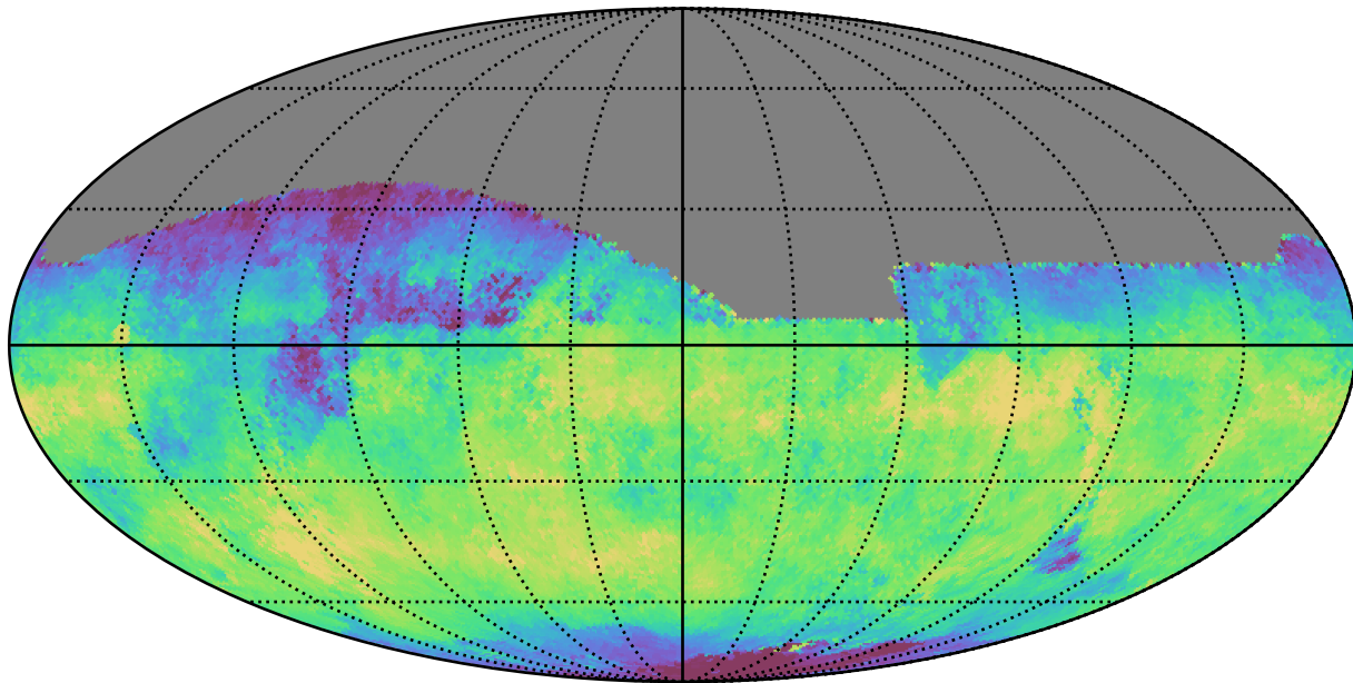
telescope_jerk_v3.5_10yrs All sky z band: Median skyBrightness
