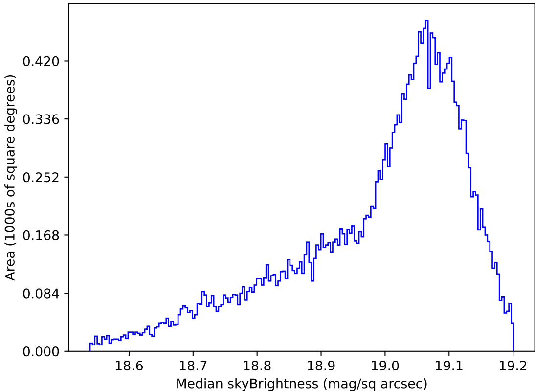
telescope_jerk_v3.5_10yrs All sky z band: Median skyBrightness
