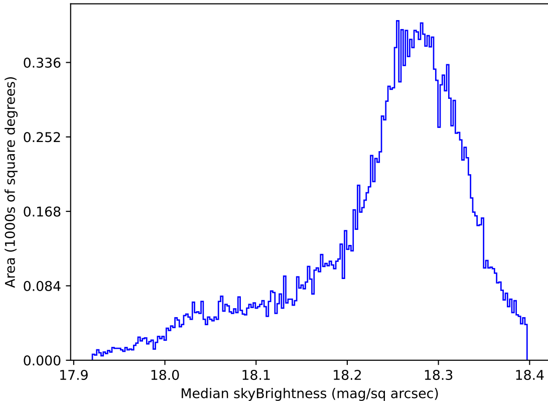
telescope_jerk_v3.5_10yrs All sky y band: Median skyBrightness
