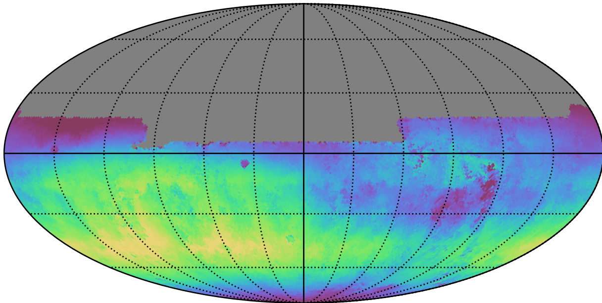
telescope_jerk_v3.5_10yrs All sky u band: Median skyBrightness
