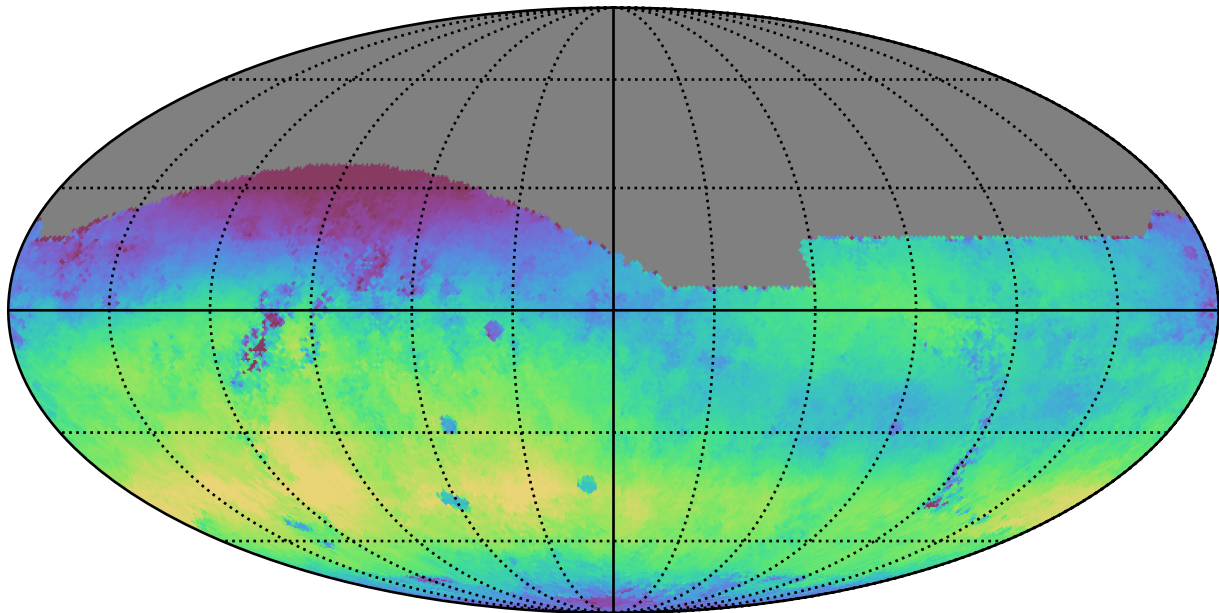
telescope_jerk_v3.5_10yrs All sky r band: Median skyBrightness
