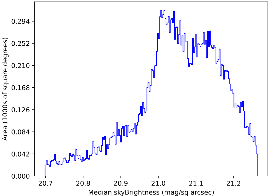
telescope_jerk_v3.5_10yrs All sky r band: Median skyBrightness
