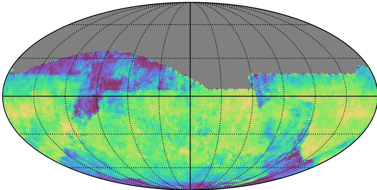
telescope_jerk_v3.5_10yrs All sky i band: Median skyBrightness
