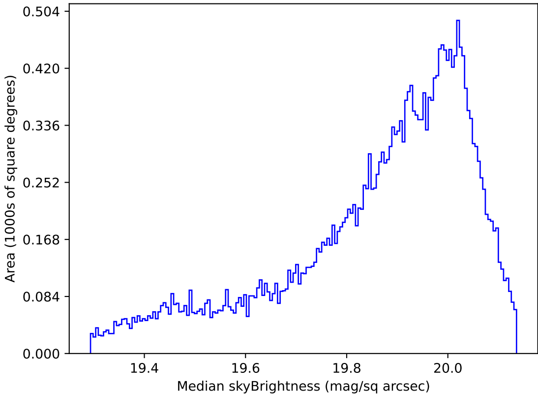
telescope_jerk_v3.5_10yrs All sky i band: Median skyBrightness
