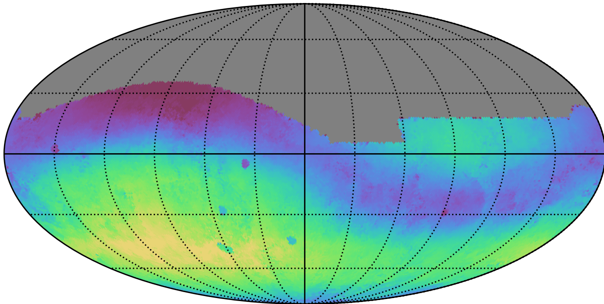
telescope_jerk_v3.5_10yrs All sky g band: Median skyBrightness
