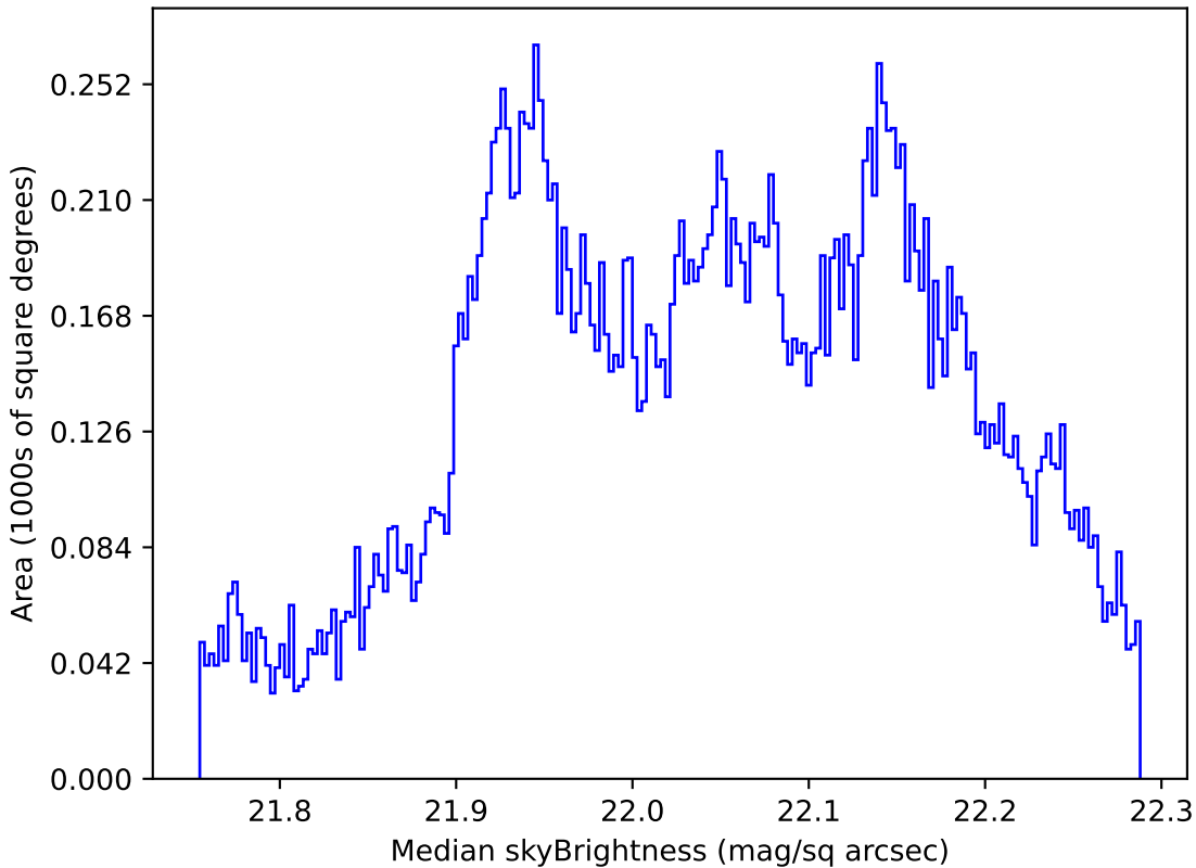
telescope_jerk_v3.5_10yrs All sky g band: Median skyBrightness
