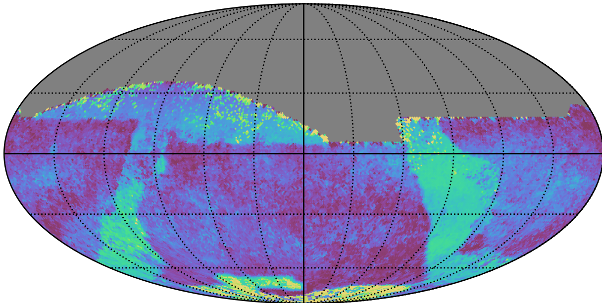
telescope_jerk_v3.5_10yrs All sky all bands: Median skyBrightness
