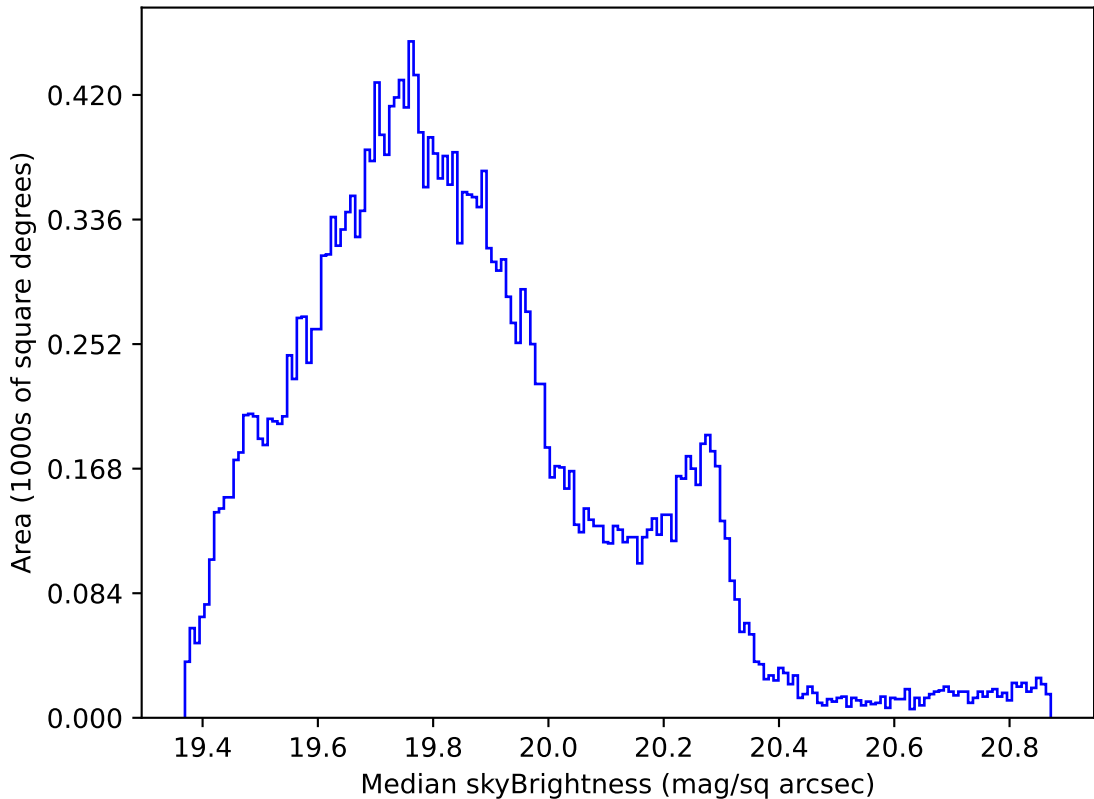
telescope_jerk_v3.5_10yrs All sky all bands: Median skyBrightness
