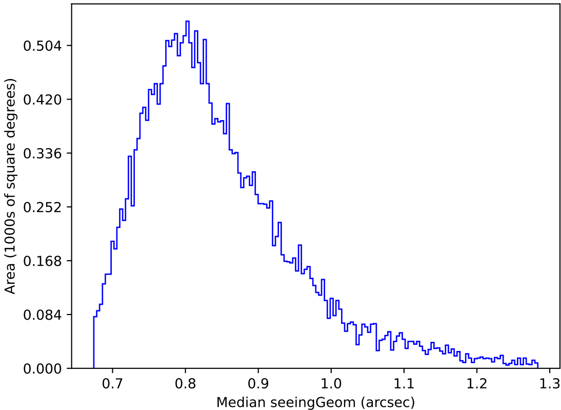
telescope_jerk_v3.5_10yrs Yr 1 z band: Median seeingGeom
