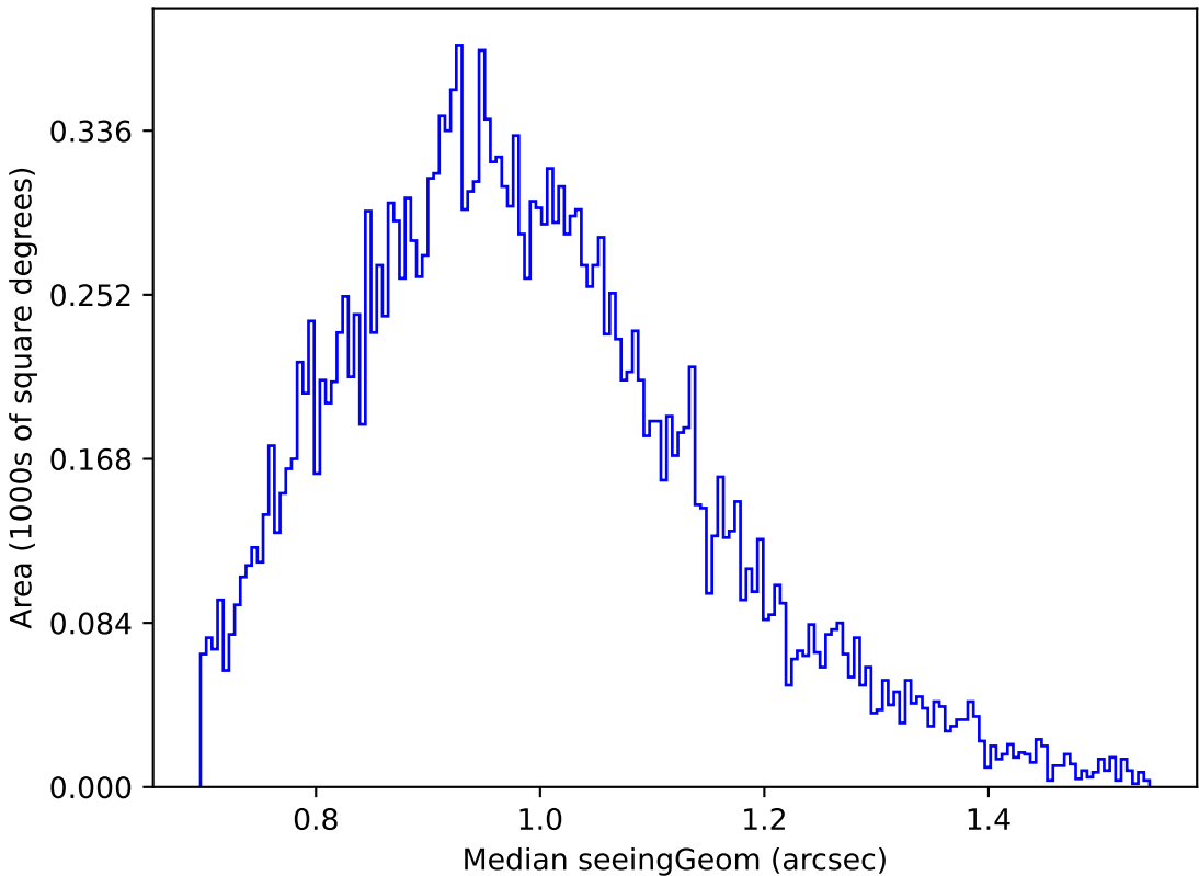
telescope_jerk_v3.5_10yrs Yr 1 u band: Median seeingGeom
