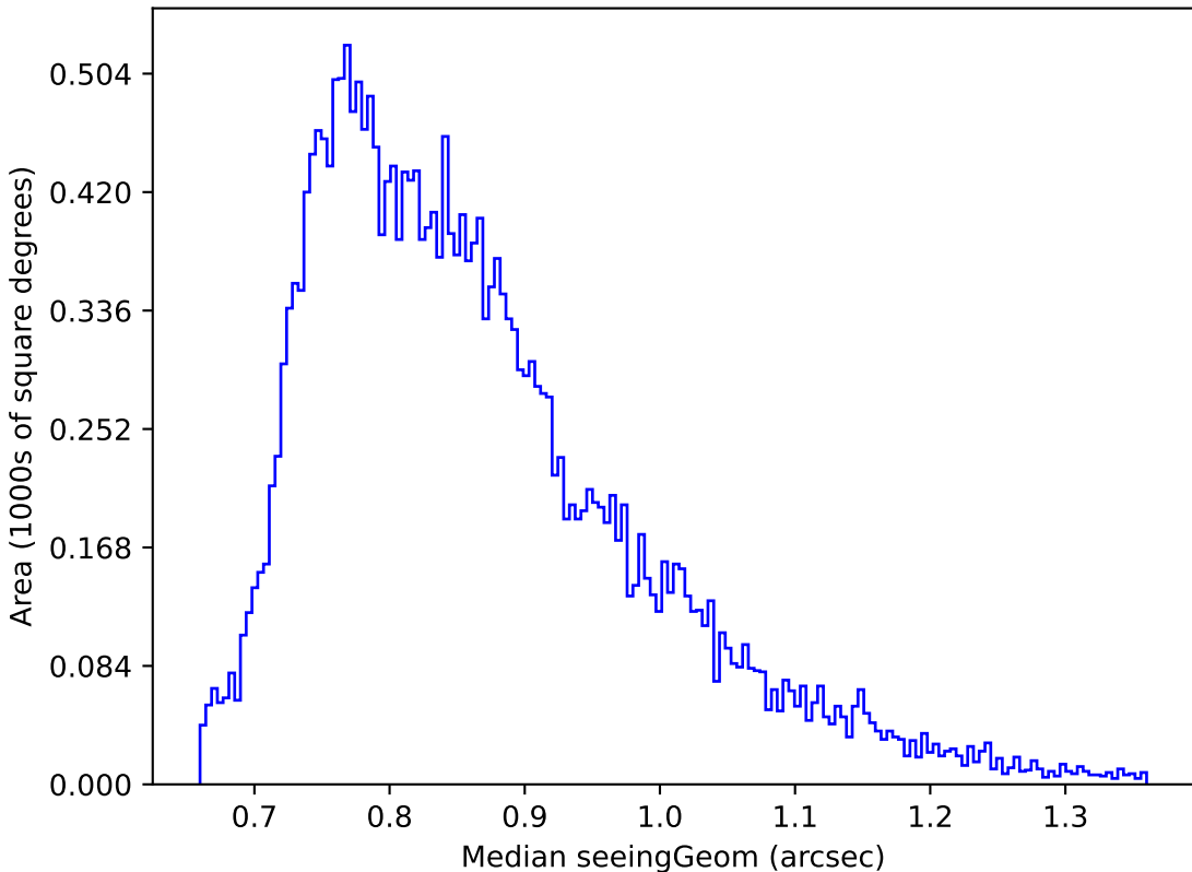
telescope_jerk_v3.5_10yrs Yr 1 r band: Median seeingGeom
