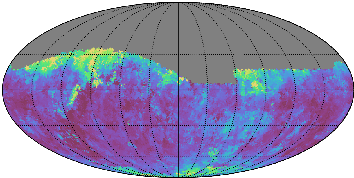
telescope_jerk_v3.5_10yrs Yr 1 i band: Median seeingGeom
