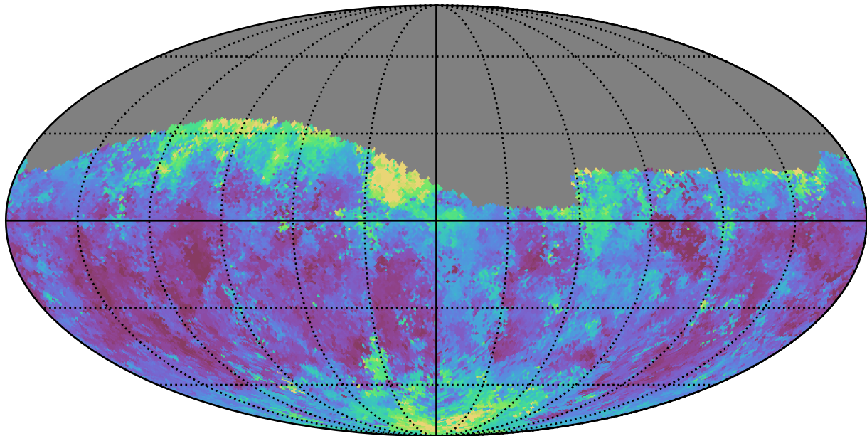
telescope_jerk_v3.5_10yrs Yr 1 g band: Median seeingGeom
