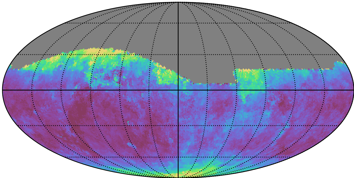
telescope_jerk_v3.5_10yrs Yr 1 all bands: Median seeingGeom
