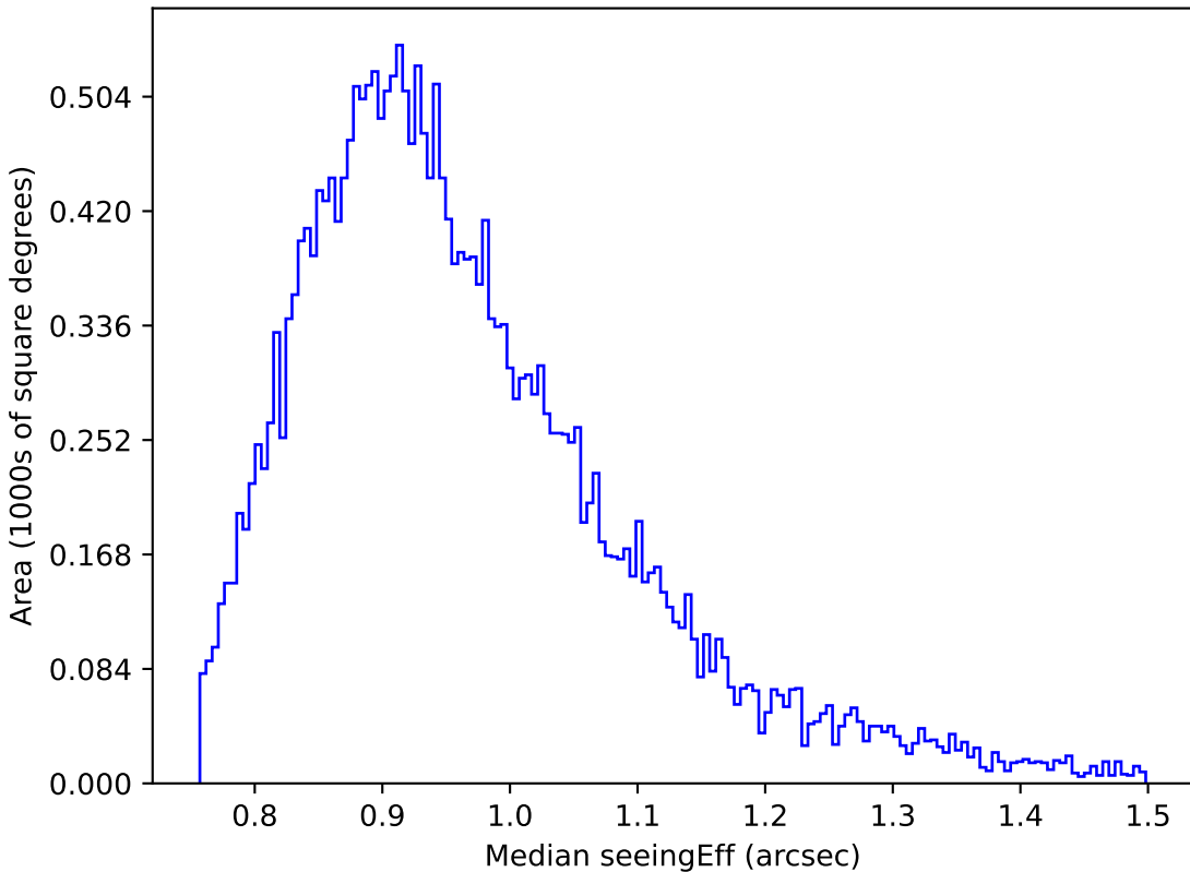
telescope_jerk_v3.5_10yrs Yr 1 z band: Median seeingEff
