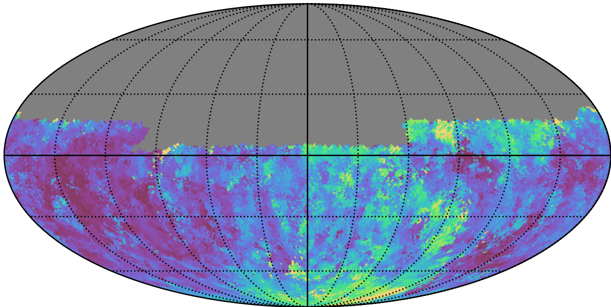
telescope_jerk_v3.5_10yrs Yr 1 u band: Median seeingEff
