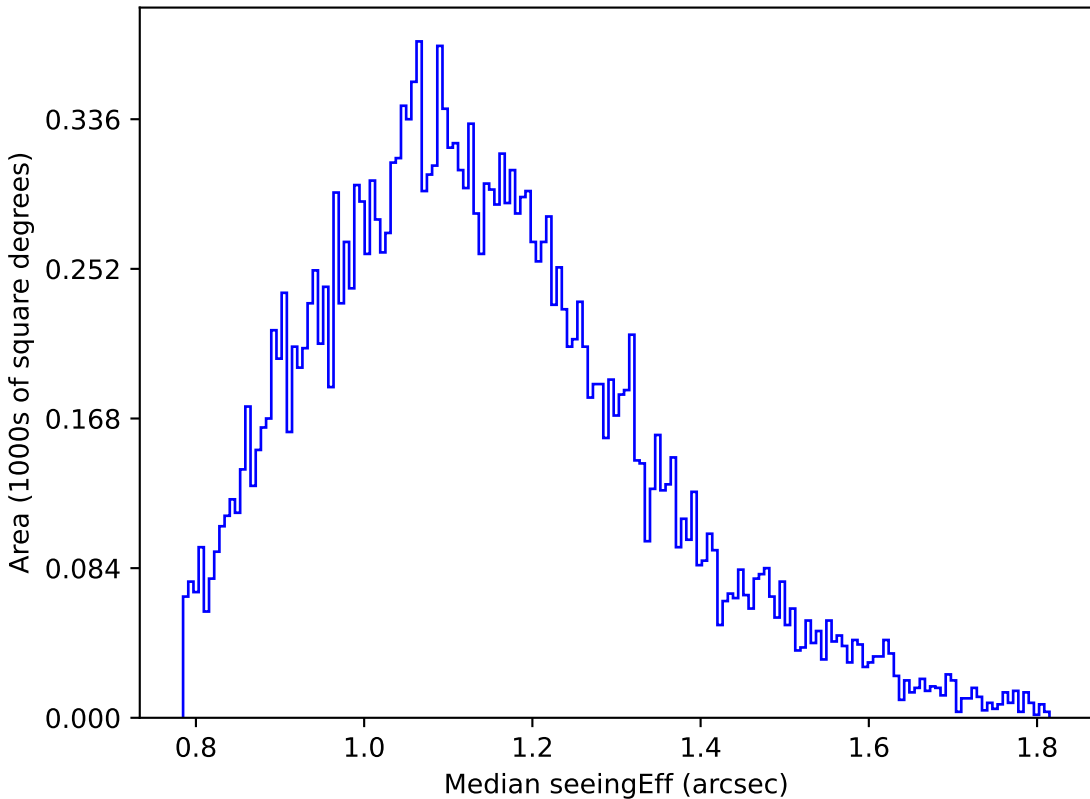
telescope_jerk_v3.5_10yrs Yr 1 u band: Median seeingEff
