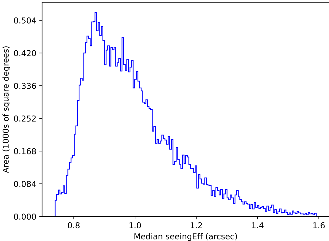
telescope_jerk_v3.5_10yrs Yr 1 r band: Median seeingEff
