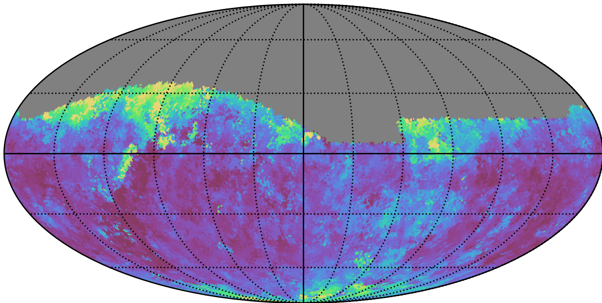
telescope_jerk_v3.5_10yrs Yr 1 i band: Median seeingEff
