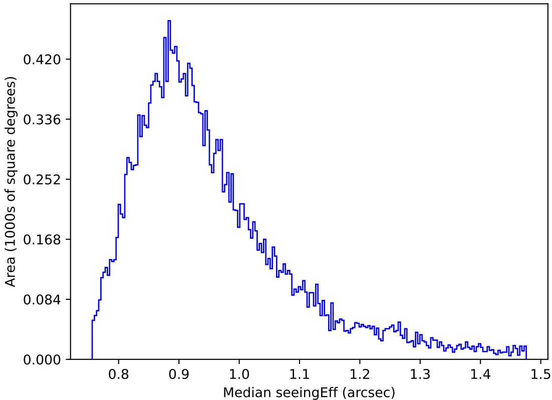
telescope_jerk_v3.5_10yrs Yr 1 i band: Median seeingEff
