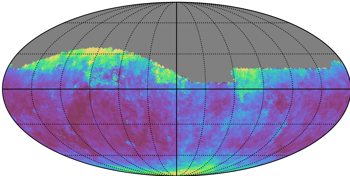
telescope_jerk_v3.5_10yrs Yr 1 all bands: Median seeingEff
