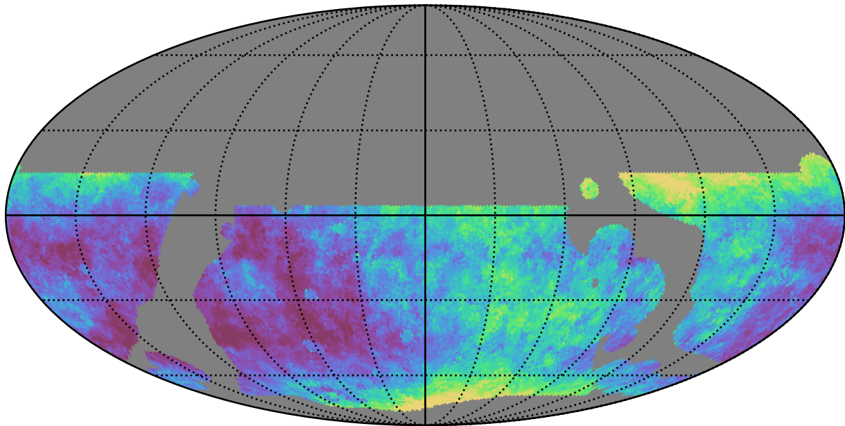
telescope_jerk_v3.5_10yrs WFD z band: Median seeingEff
