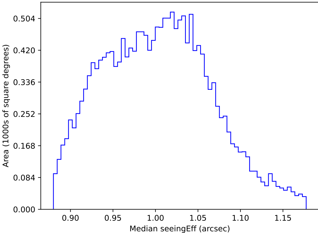
telescope_jerk_v3.5_10yrs WFD z band: Median seeingEff
