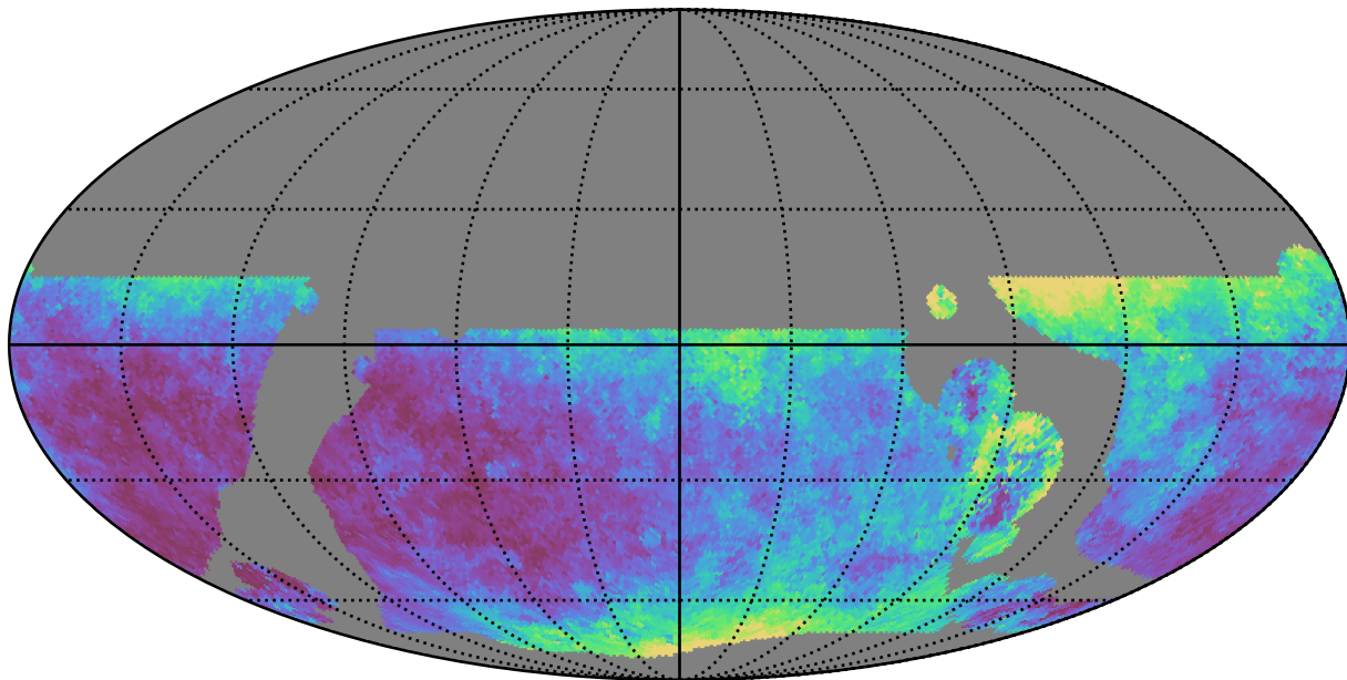
telescope_jerk_v3.5_10yrs WFD y band: Median seeingEff
