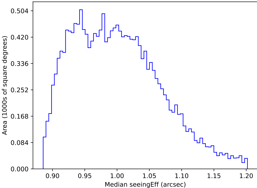
telescope_jerk_v3.5_10yrs WFD y band: Median seeingEff
