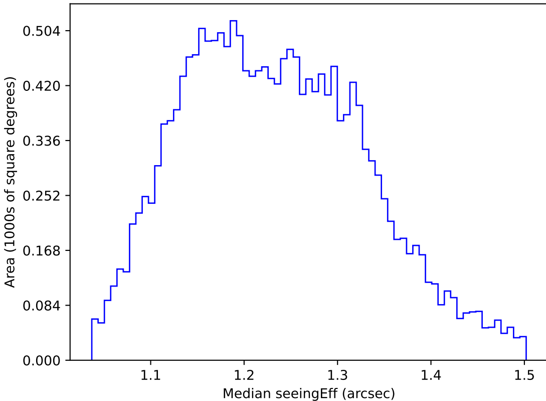
telescope_jerk_v3.5_10yrs WFD u band: Median seeingEff
