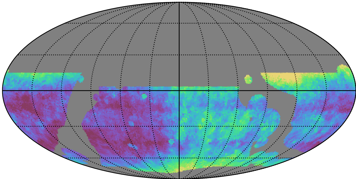
telescope_jerk_v3.5_10yrs WFD r band: Median seeingEff
