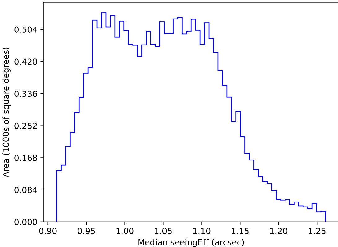
telescope_jerk_v3.5_10yrs WFD r band: Median seeingEff
