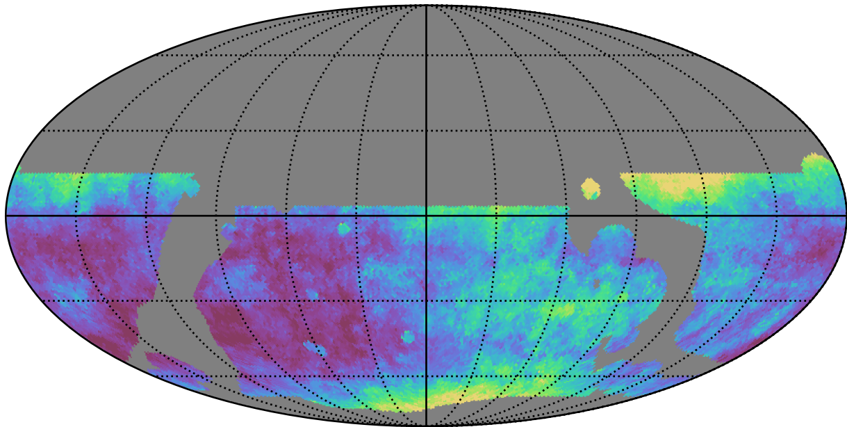
telescope_jerk_v3.5_10yrs WFD i band: Median seeingEff
