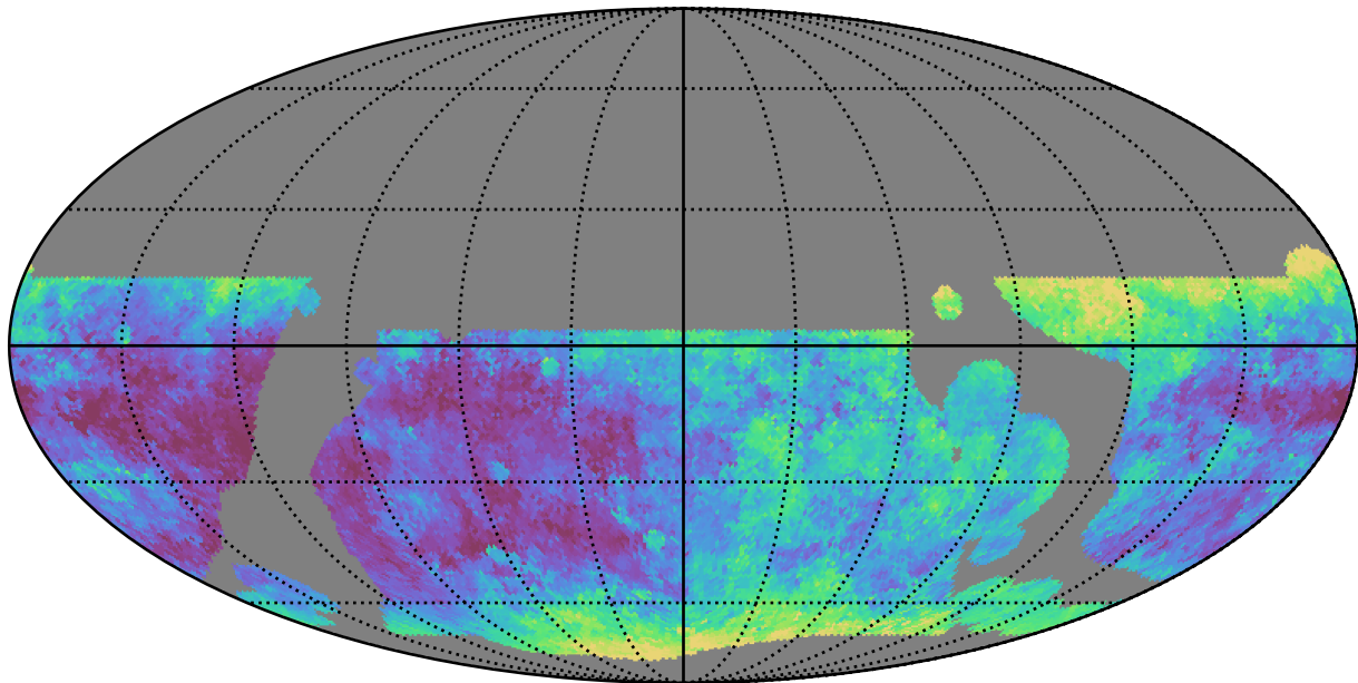
telescope_jerk_v3.5_10yrs WFD g band: Median seeingEff
