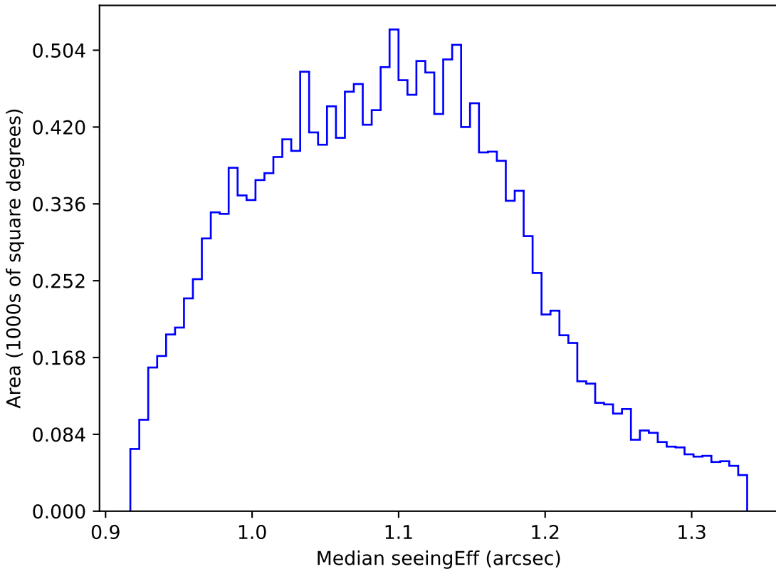
telescope_jerk_v3.5_10yrs WFD g band: Median seeingEff
