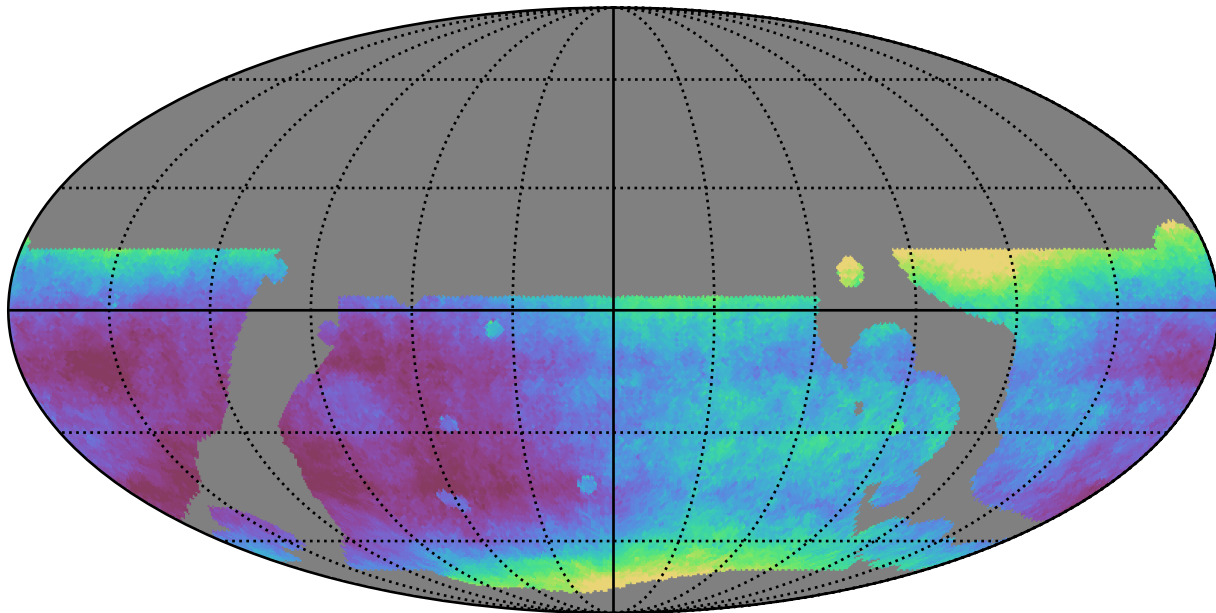
telescope_jerk_v3.5_10yrs WFD all bands: Median seeingEff
