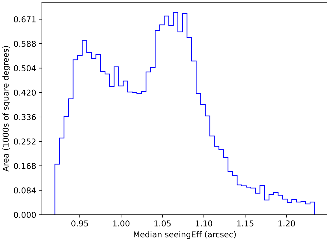
telescope_jerk_v3.5_10yrs WFD all bands: Median seeingEff
