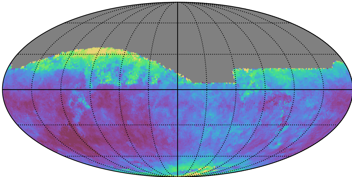
telescope_jerk_v3.5_10yrs All sky z band: Median seeingEff
