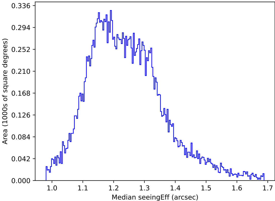
telescope_jerk_v3.5_10yrs All sky u band: Median seeingEff
