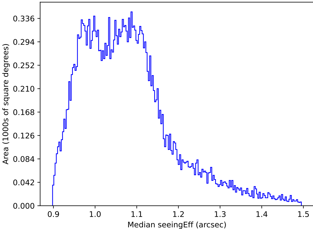
telescope_jerk_v3.5_10yrs All sky r band: Median seeingEff
