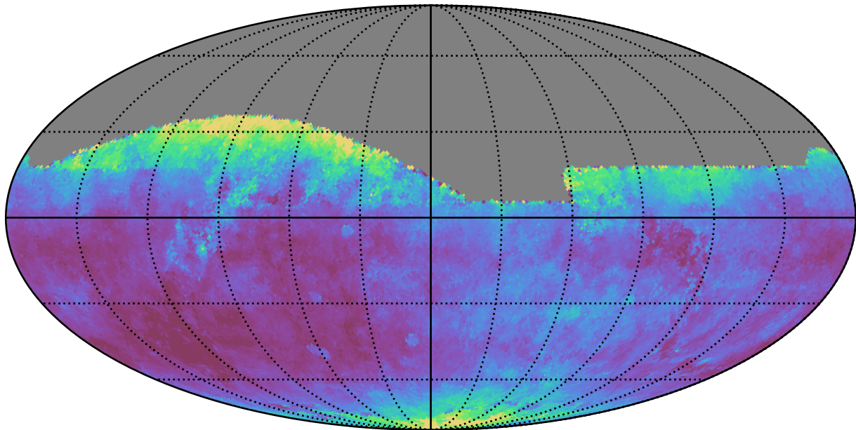
telescope_jerk_v3.5_10yrs All sky i band: Median seeingEff
