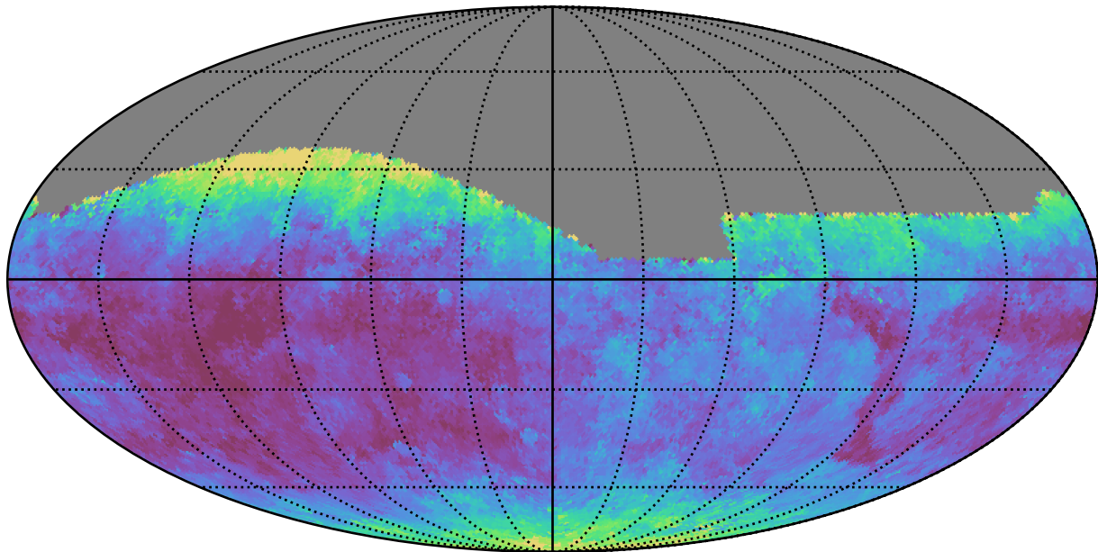
telescope_jerk_v3.5_10yrs All sky g band: Median seeingEff
