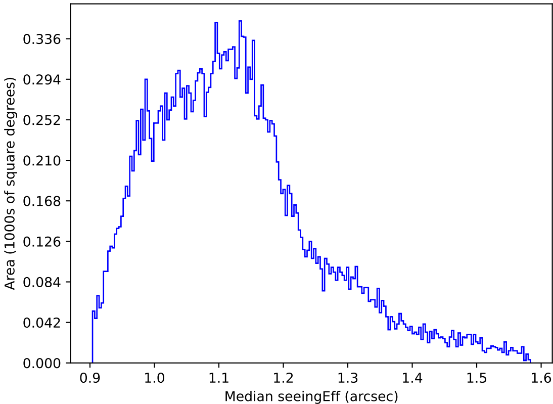
telescope_jerk_v3.5_10yrs All sky g band: Median seeingEff
