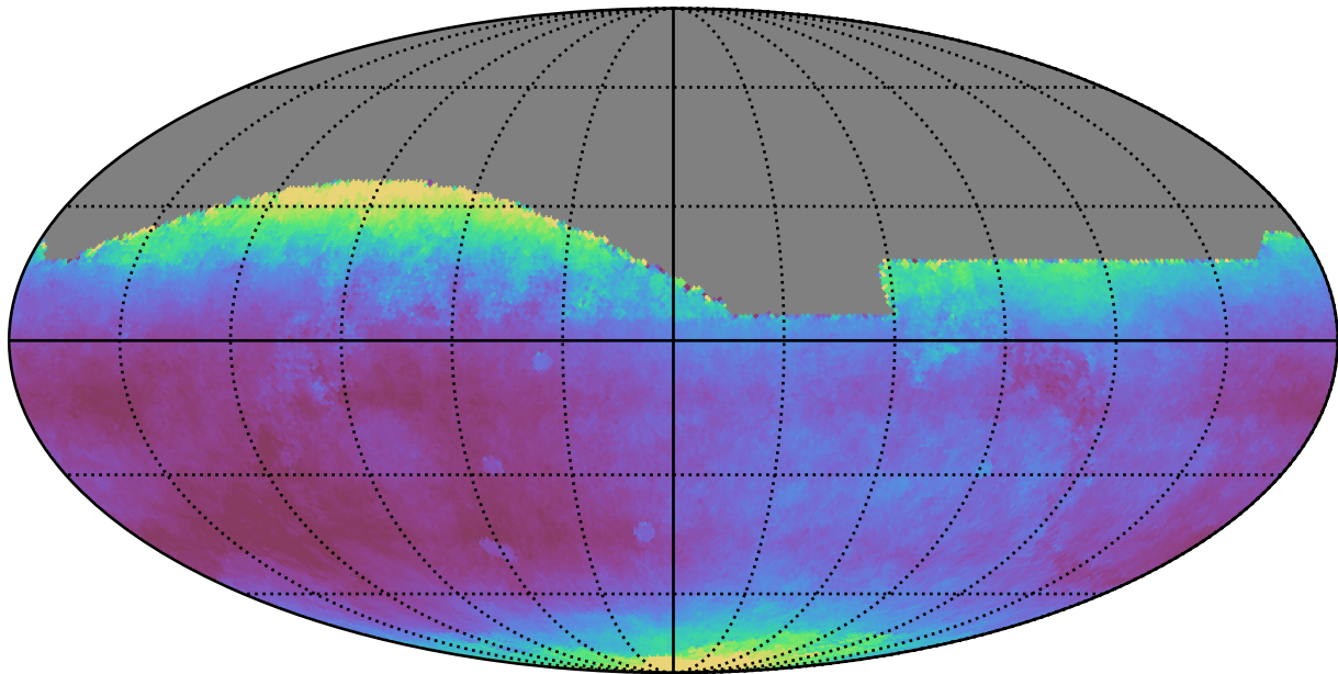
telescope_jerk_v3.5_10yrs All sky all bands: Median seeingEff
