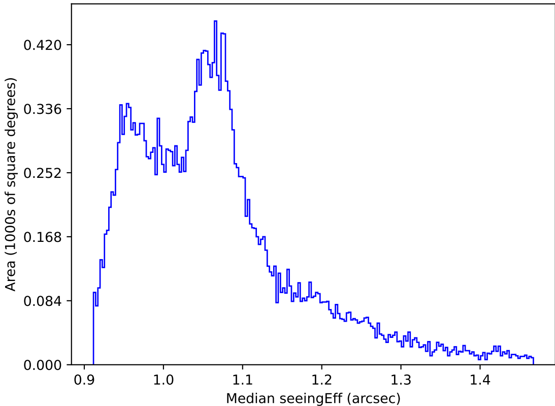
telescope_jerk_v3.5_10yrs All sky all bands: Median seeingEff
