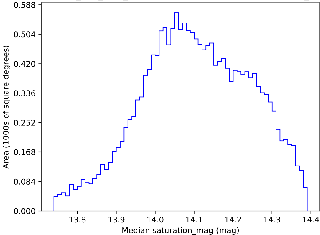
telescope_jerk_v3.5_10yrs WFD z band: Median saturation_mag
