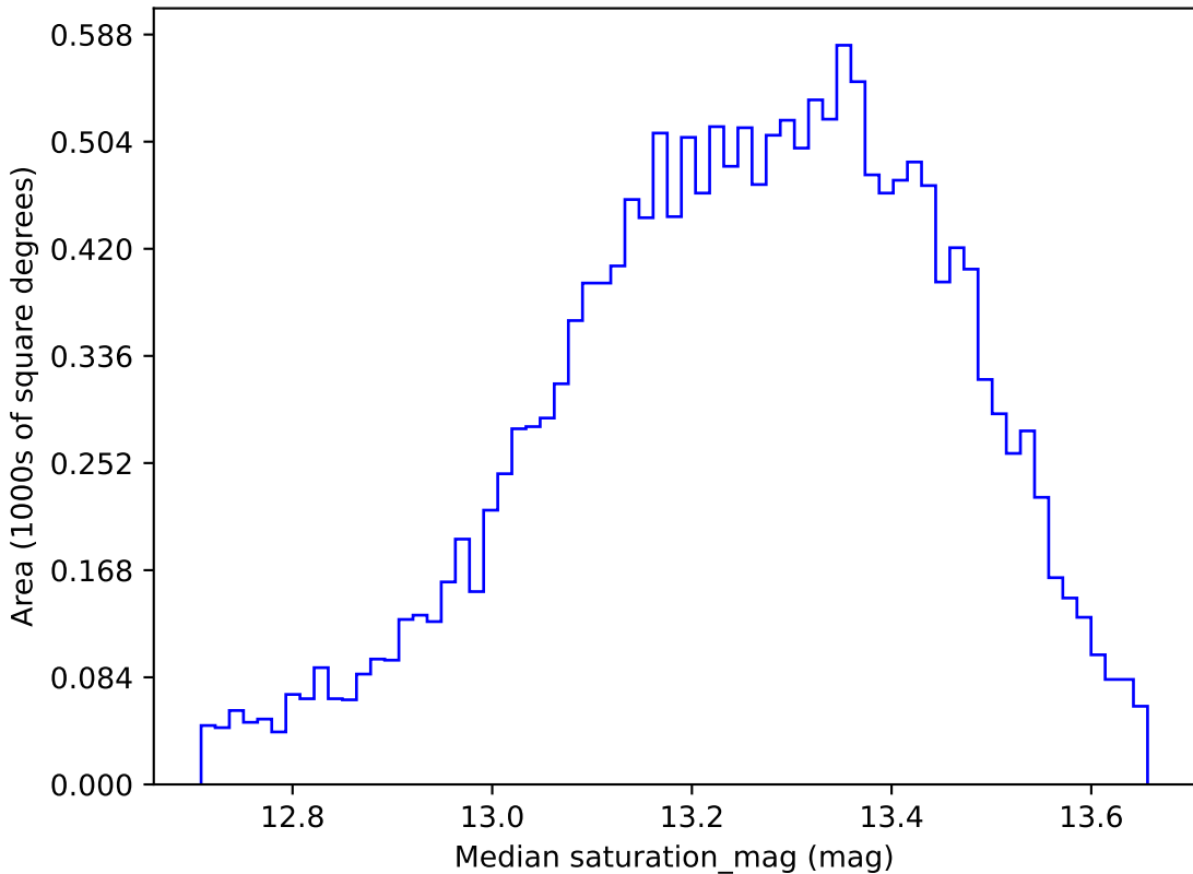
telescope_jerk_v3.5_10yrs WFD u band: Median saturation_mag
