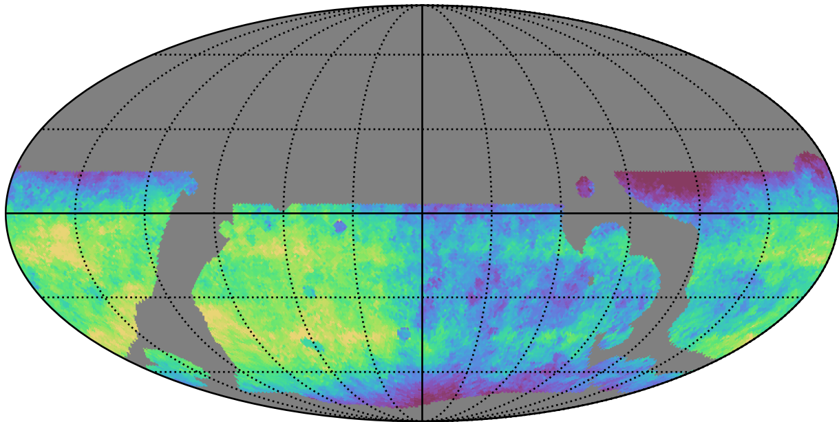
telescope_jerk_v3.5_10yrs WFD r band: Median saturation_mag
