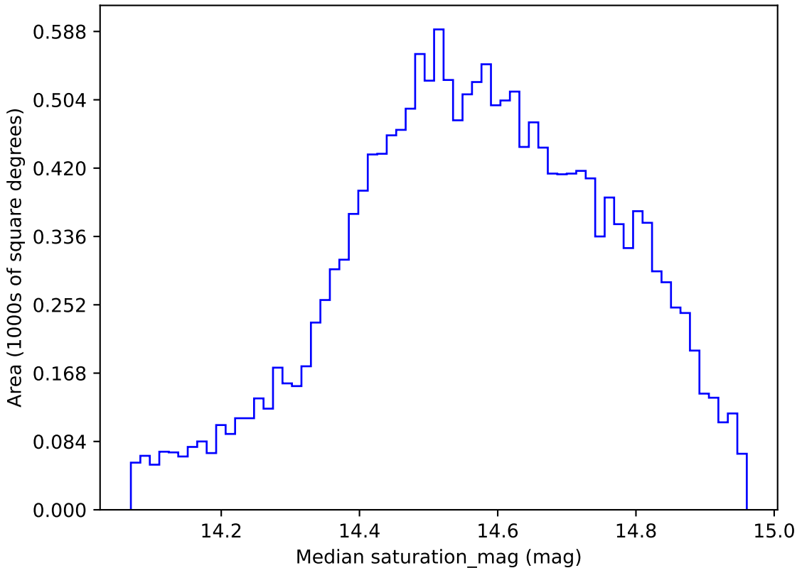
telescope_jerk_v3.5_10yrs WFD g band: Median saturation_mag
