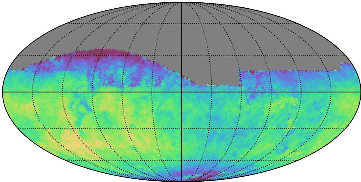
telescope_jerk_v3.5_10yrs All sky z band: Median saturation_mag
